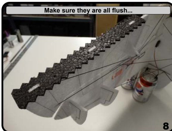
And the shorter one to the elevator trailing edge
