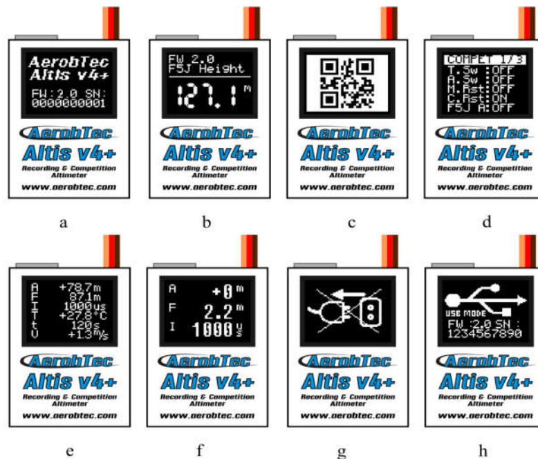
Fig 7: Various screens: a) Initialization screen b) F5J screen c) QR code screen d) Settings screen e) User defined screen with 6 lines f) User defined screen with 3 lines g) Do not disconnect screen h) USB mode screen
