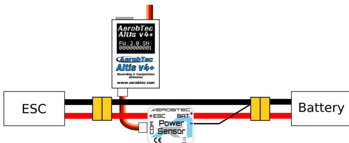
Fig 18: Power sensor connection
