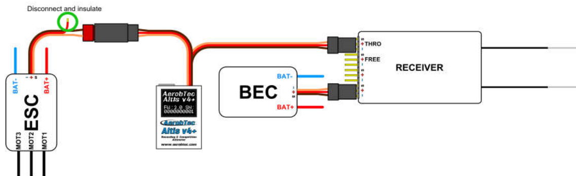
Fig 4: Connection of Altis v4+ with external BEC
