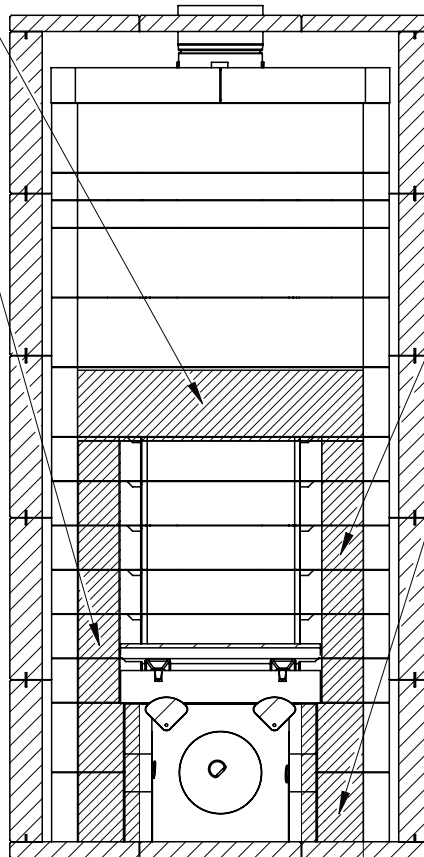
SECTION F-F SCALE 1 : 14
