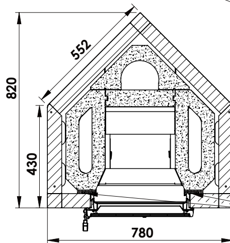
SECTION C-C SCALE 1 : 16
