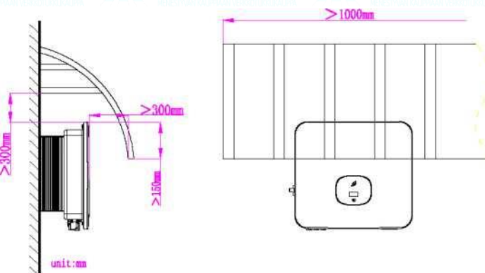
Fig 5.6 Sunshade
