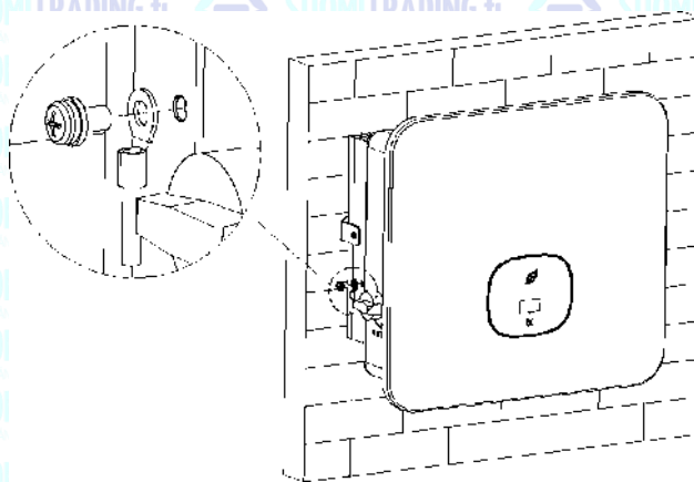
Fig 6.1 Grounding diagram
